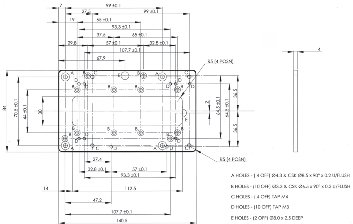
FIXING POSITIONS OF BACKPLATE SUPPLIED WITH MOUNT
